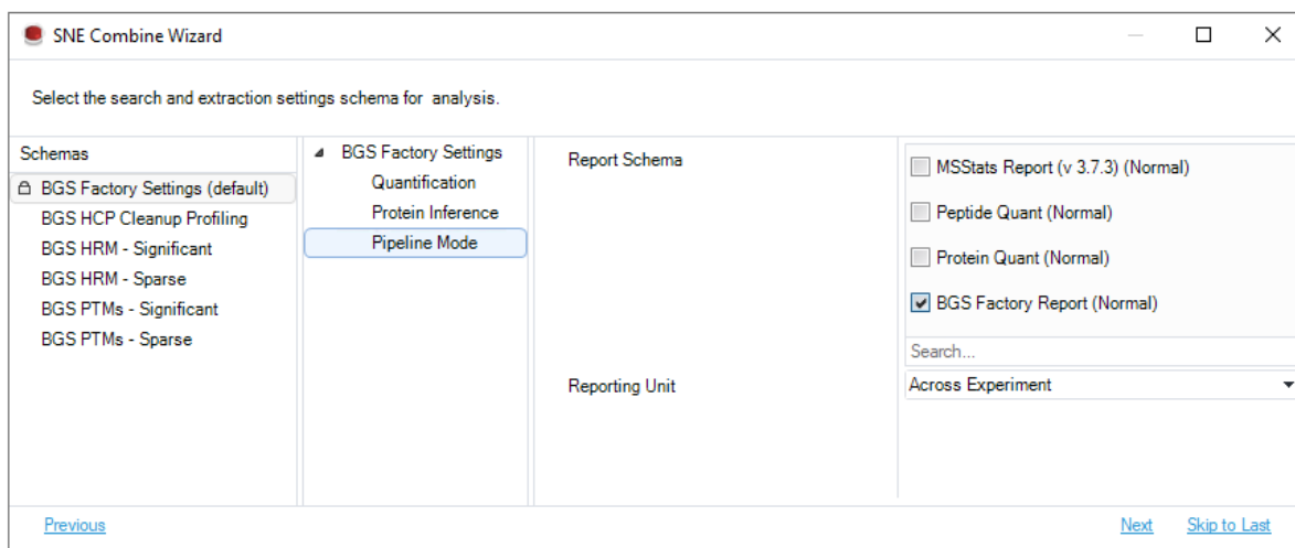
Figure 46. The SNE Combine Wizard guides through the parameters that are recalculated during multiple SNE files merging.
