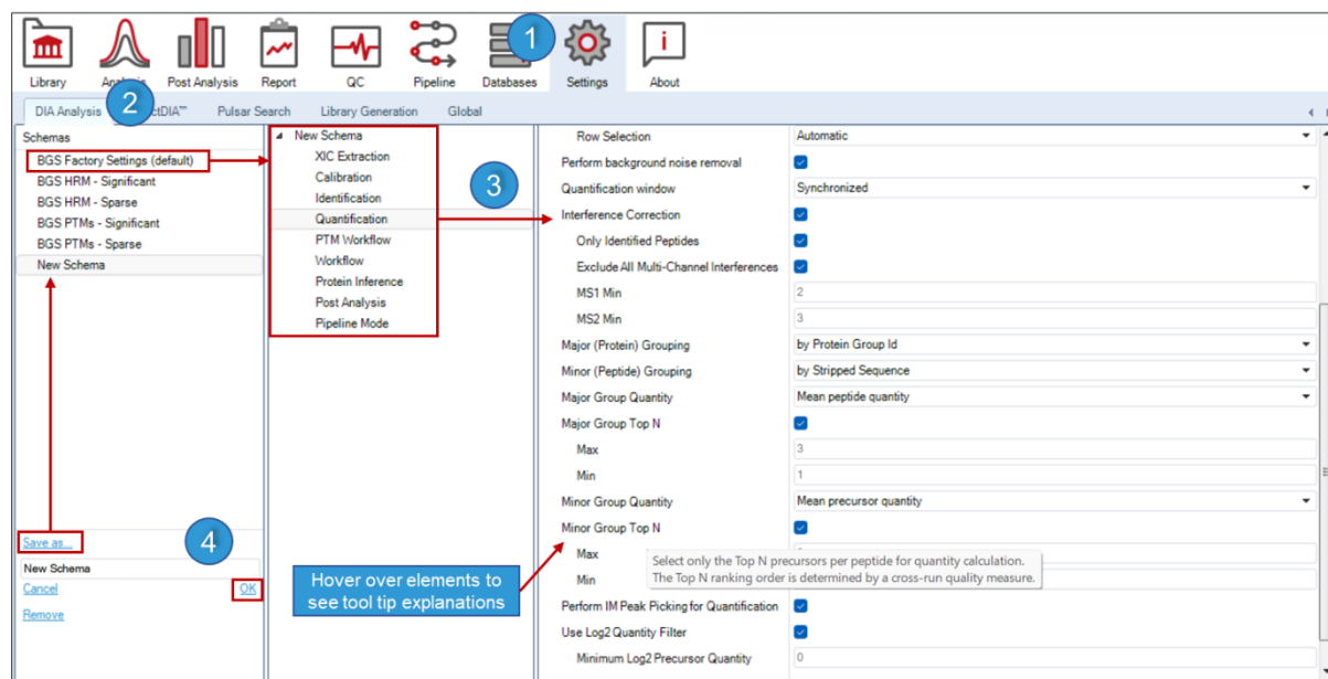
Figure 51. Make a custom schema for your analysis. The new schemas will be available during the subsequent analysis set-ups.
