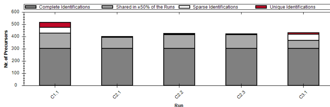
Figure 86. The upper-panel plot under the "Run Identifications" node shows the number of precursors per run and their completeness.
