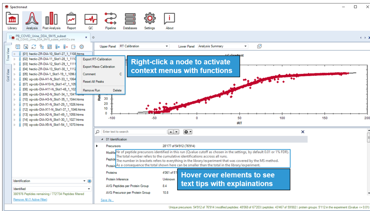
Figure 4. Spectronaut contains tooltips and menus when you hover over some elements or right-click on them.
