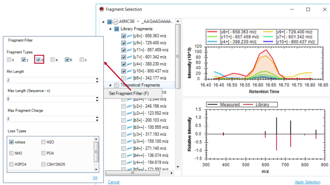
Figure 33. Refine your library while reviewing your analysis. You can, for example, use different ion series (z-ions) by adding them into the fragment tree and selecting them. A preview of how the XIC looks with the current selected ions is shown on the right. You can also look at how individual ions XICs appear by selecting individual ions.
