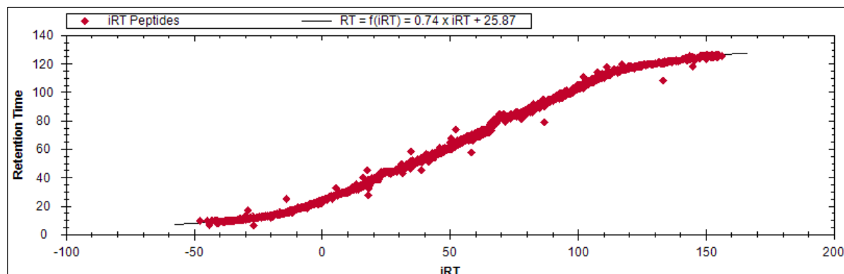
Figure 54. iRT Calibration Chart showing the non-linear transformation from library iRT to actual predicted retention times. The chart is shown after extended non-linear calibration has been performed. The extended calibration allows you to correct even small gradient fine-structure fluctuations to get the most accurate retention time prediction for your library.
