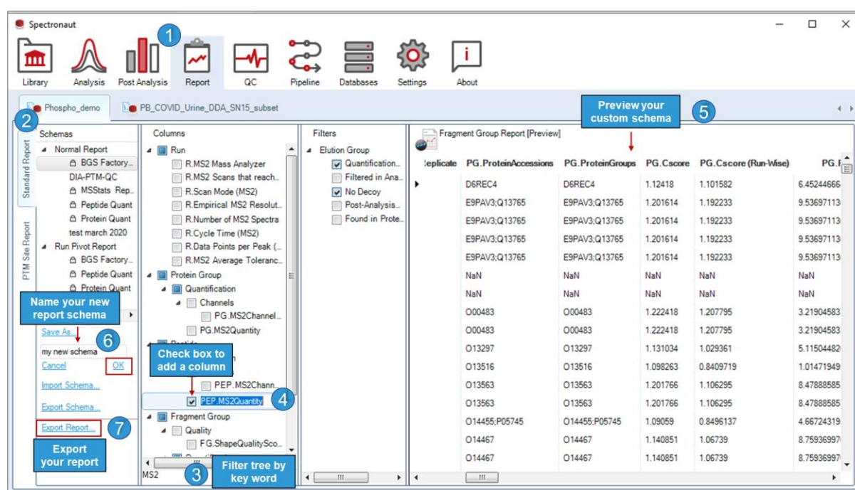
Figure 41. Report Perspective. The figure shows the process of customizing a Normal Report schema and exporting the data. Detailed explanation of the headers can be found by hovering over them or in Appendix 8. Most Relevant Report Headers
