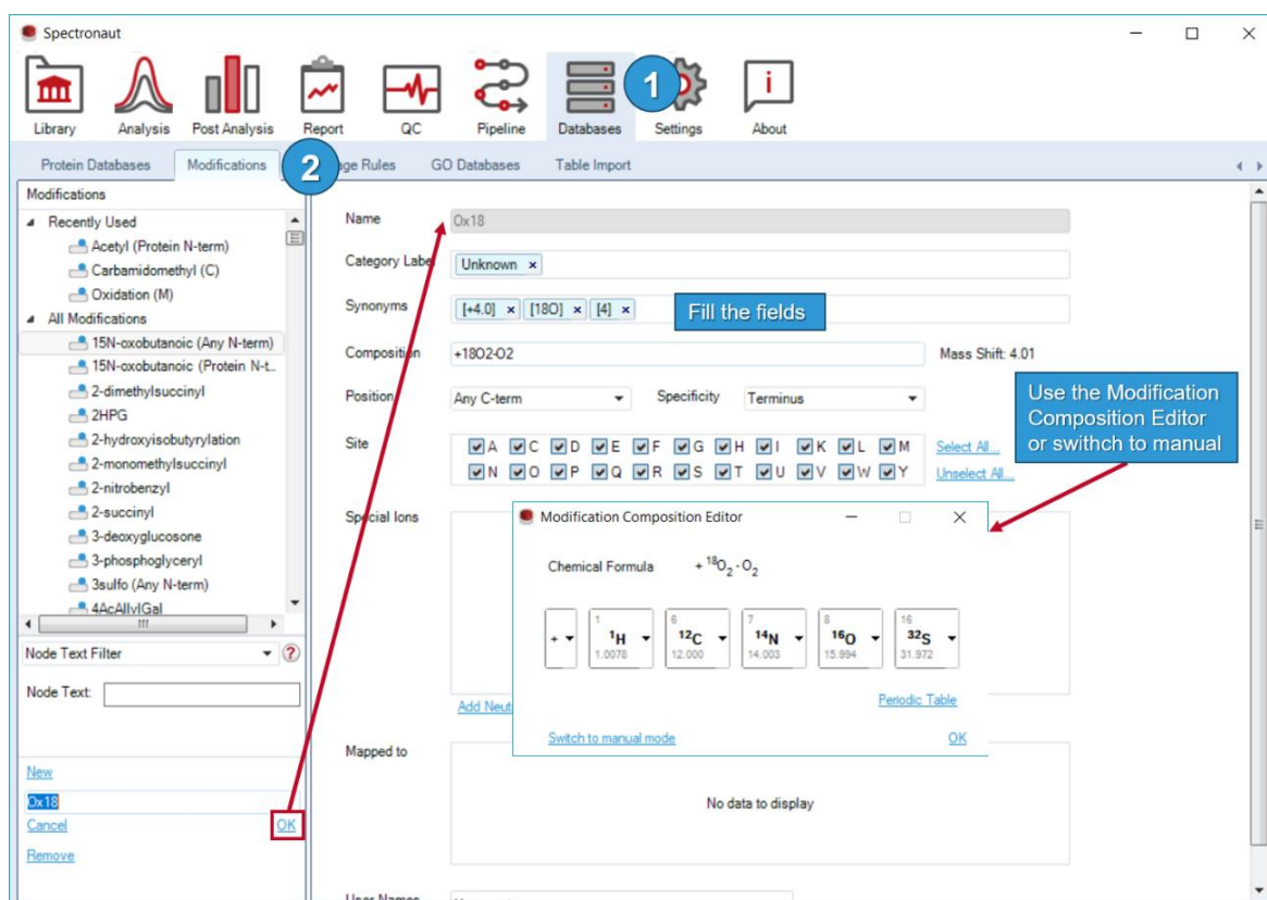
Figure 49. Adding a new modification to the database.
