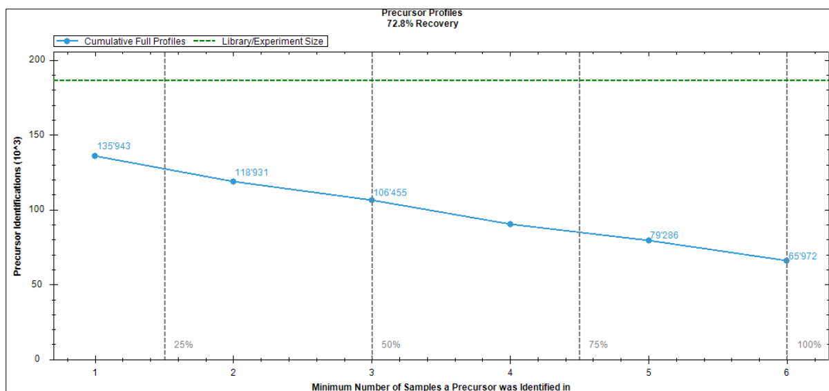
Figure 88. The upper plot under the "Data Completeness" node shows number of cumulative full profiles. The blue line represents the decline of full profiles. The plot shows in an easy way how many precursors were identified in a given percentage of all runs. For example, in the first 3 runs (50% of the runs), 106.455 precursors were identified in all of those 3 runs. As with many other plots you can change the context to display the data completeness on precursor, peptide, protein-group or protein level.
