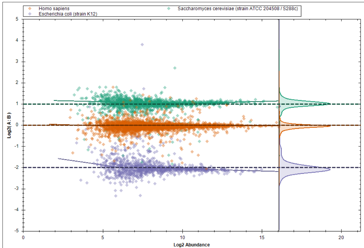
Figure 105. The LFQBench plot for mixed proteomes of three organisms. The Y-axis (log2Ratio) shows the ratios of the mixed proteomes based on experimental data. The expected ratios (dashed lines) can be set by right-clicking on the plot. The distributions on the right side of the plot show how the experimental diverge from the expected ratios. The X-axis represents protein abundance (log2-transformed).
