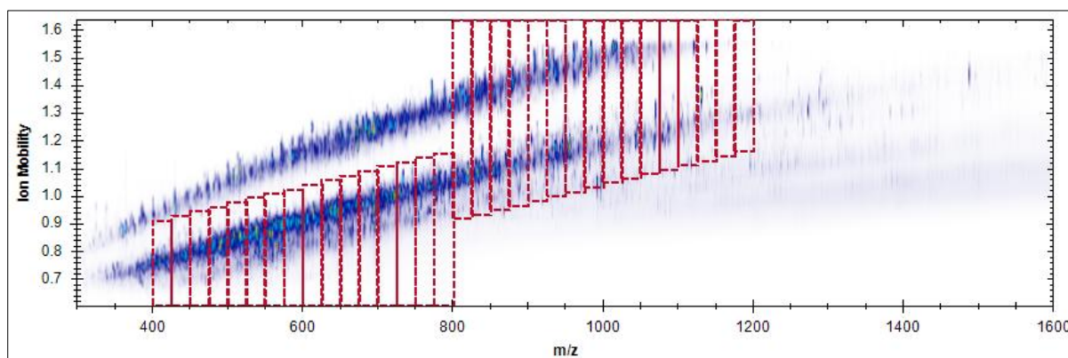
Figure 65. The Ion Mobility Overview plot shows the ion mobility dimension in function of m/z values. The red lines show consecutive DIA boxes. Their overlay with registered MS1 signal could be used for DIA method optimization and validation.
