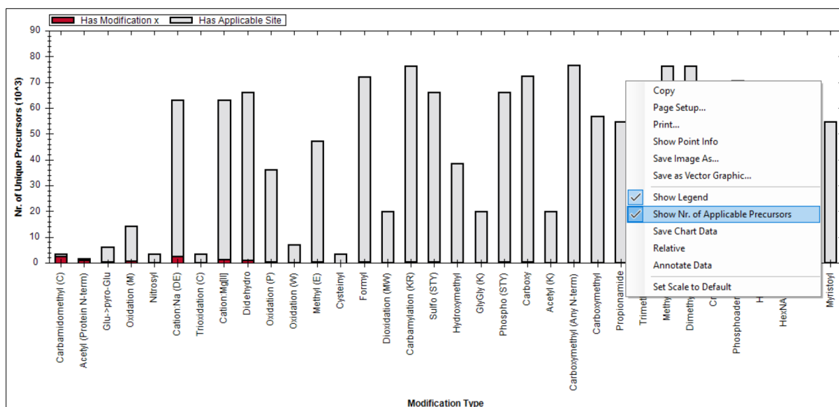
Figure 100. By right-clicking, the number of unique precursors that contain possible sites for each modification can be added to the Detected Modifications plot.
