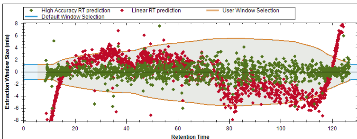
Figure 56. The XIC Extraction Width plot gives insight into your gradient stability and the overall accuracy of your library's iRT values. The blue and the orange lines show the window selections as suggested by Spectronaut (blue) and as set by the user (orange → correction factor in the settings). These extraction window widths (y-axis) change over time (x-axis) based on gradient stability and iRT accuracy. The red dots show your library's iRT accuracy assuming a linear iRT to RT transformation. The green dots show the iRT accuracy using the extended non-linear iRT to RT transformation. The latter one is used for the actual analysis.
