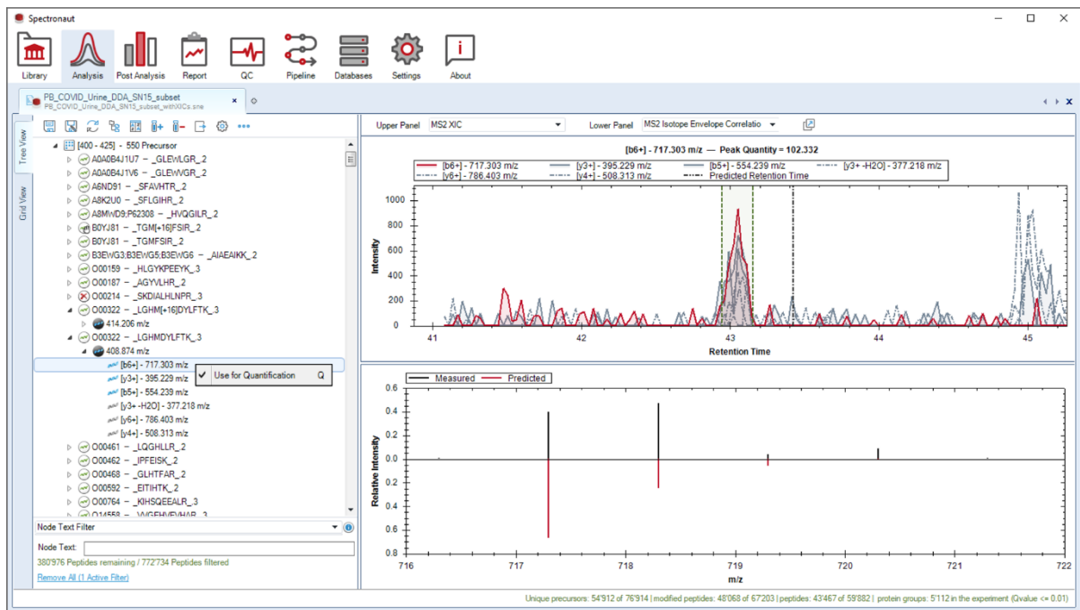
Figure 32. Manually define interfering fragment ions or manually accept fragment ions for quantitation that were defined as interferences by Spectronaut.
