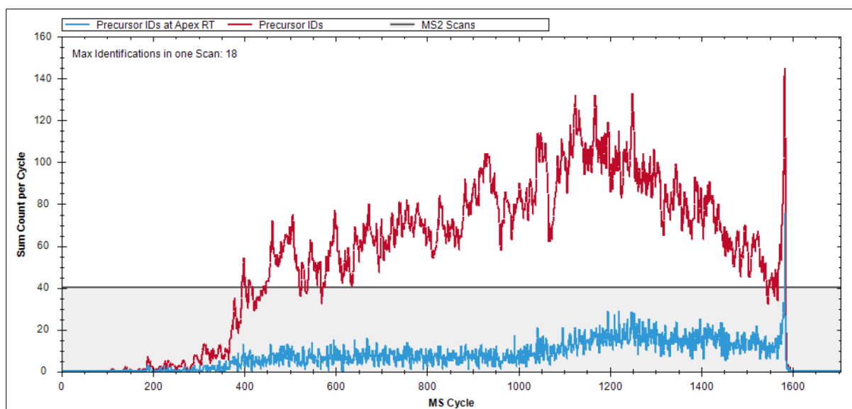
Figure 66. The Identifications Per Cycle plot shows the Precursor IDs at Apex RT (blue) and Precursor IDs (red) across all MS cycles.
