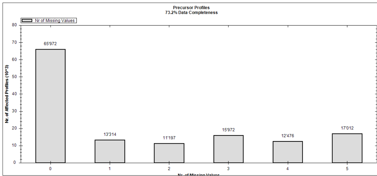
Figure 89. The lower plot under the "Data Completeness" node shows the histogram of missing values. In this plot, about 66.000 precursors did not have any missing values and were identified in every run (this is equivalent to the last data point in Figure 88) while about 13.300 precursors had one missing value and so forth. The last bar represents the number of single-hit precursors. These are the precursors that were only identified in one single run (hence they were only identified in 1 out of 6 runs in this case). As with many other plots you can change the context to show you the missing values on precursor, peptide, protein-group or protein level.
