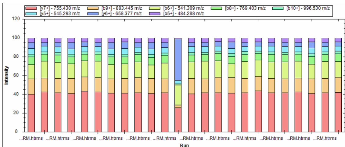
Figure 81. The MS2 Intensity alignment for a peptide containing 8 fragment ions. Each fragment ions relative intensity compared to the total peak height is indicated using a differently colored bar. The peptide was targeted in 24 runs. An inconsistent signal can be easily identified due to the sudden change in the color pattern.
