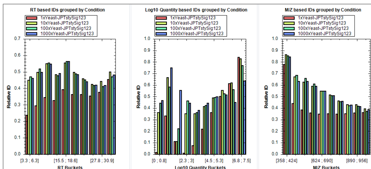
Figure 103. Binned Identification plot shows relative ID plotted for Retention Time buckets, Log10 Quantity buckets and m/z buckets. Data is grouped by the condition which, upon right clicking, could be changed to run or fraction.
