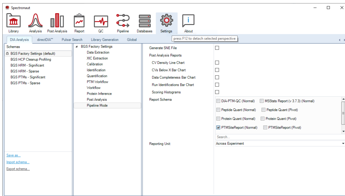
Figure 47. DIA Analysis Pipeline Mode Settings. Define which results from the Pipeline Perspective should be saved.
