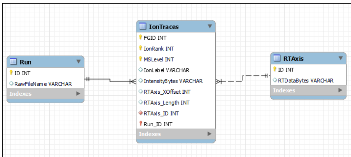
Figure 114 XIC export database schema. The XIC db can be exported on a per-experiment basis. The exported database consists of 3 SQL tables.
