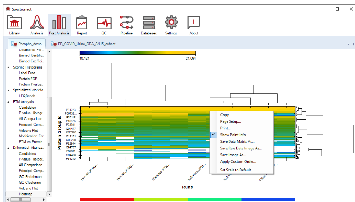
Figure 37. Heatmap with clustering in both rows and columns. The heatmap is built using the set of confidently identified datapoints. By right-clicking on the plot you can perform several actions, such as Save Image As, export the data matrix, or modify the scaling.
