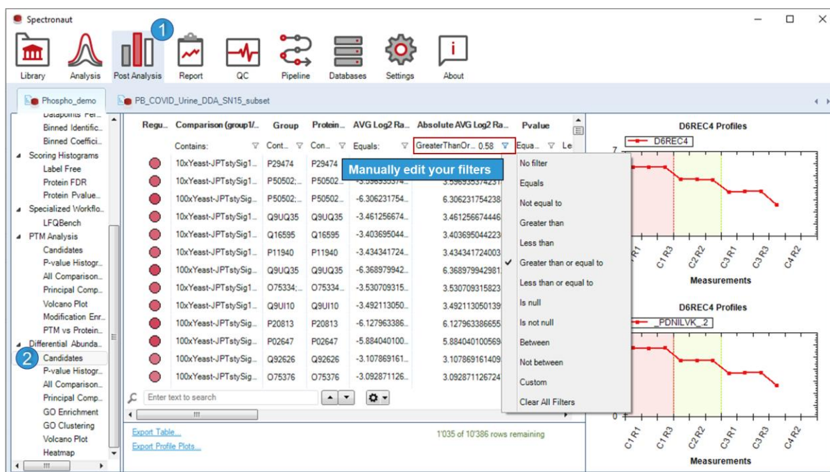
Figure 34. Post Analysis Perspective. Several summaries, tables, and plots are available as you navigate through the nodes in the tree. In the figure, you can visualize the Candidates list. You can modify your candidate set by filtering directly on this table. The default applied filters are a 1.5-fold change and a q-value of 0.05.
